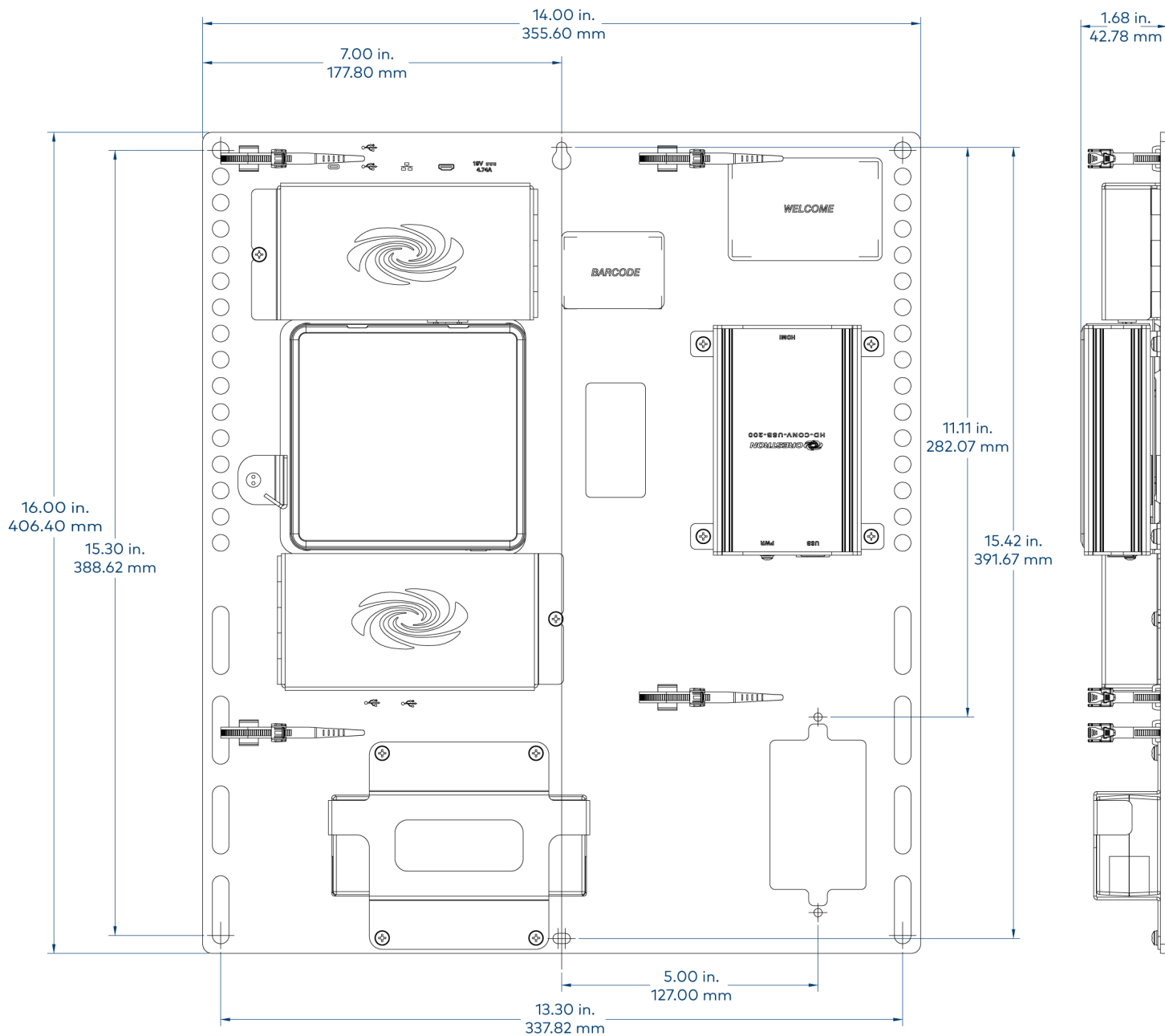
UC-BRKT-100-SD-ASSY
